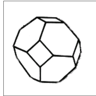
Abb. 3: Kubooktaeder
