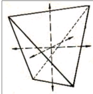
Abb. 2: Tetraeder
