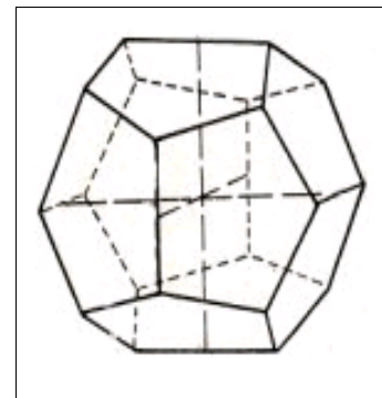
Abb. 6: Pentagondodekaeder
