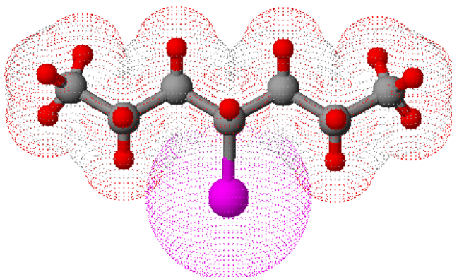
4-Brom-Heptan =
