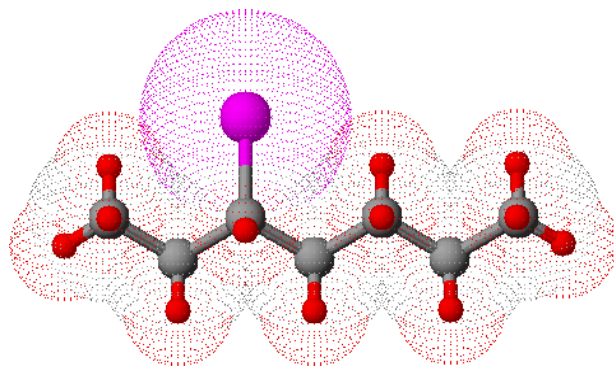
3-Brom-Heptan =
