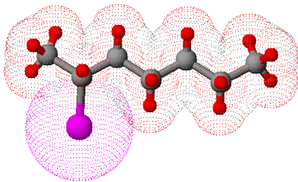
2-Brom-Heptan =
