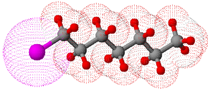
1-Brom-Heptan =
